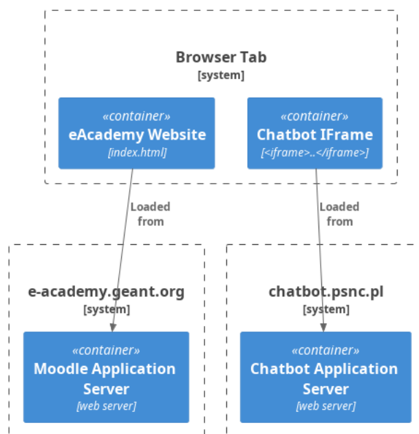
Figure 2: Chatbot components within the GÉANT eAcademy environment
